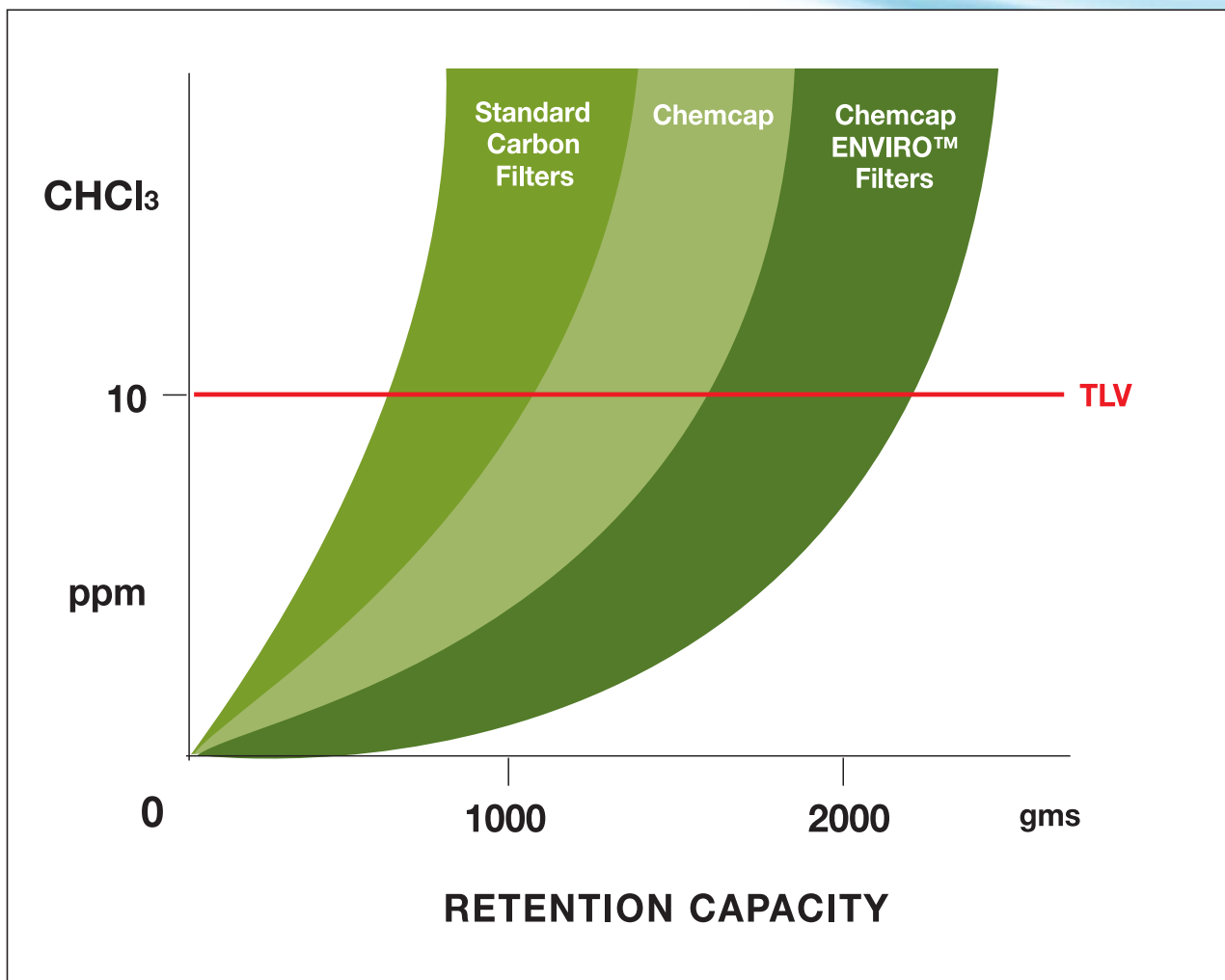
Graph shows retention for an OS Chemcap Enviro filter (size F4)
